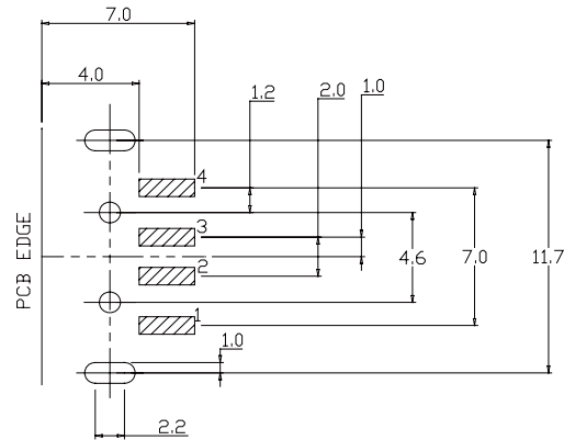
COMPONENT SIDE (PCB LAYOUT)
